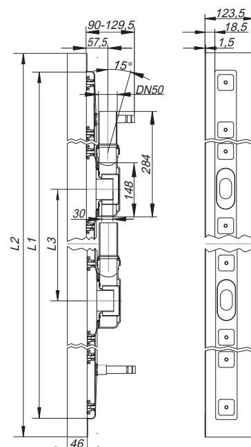
Duschrinne CeraLine Plan W Duo 1100 – 2000
