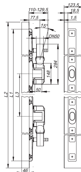
Duschrinne CeraLine W Duo 800 – 1000
