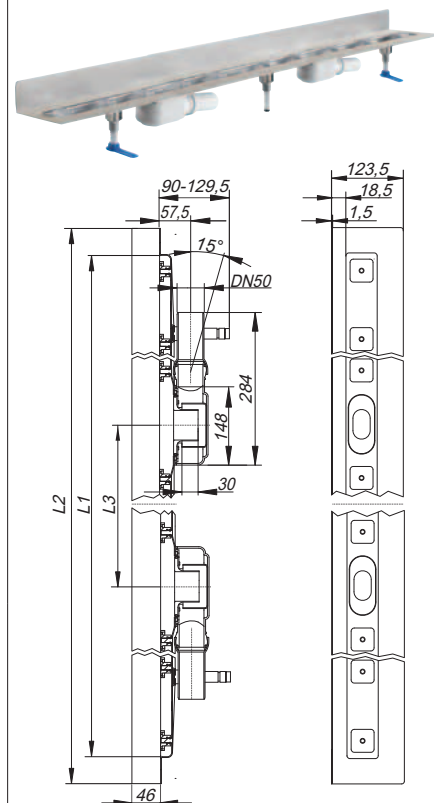
Duschrinne CeraLine Plan W Duo 800 – 1000
