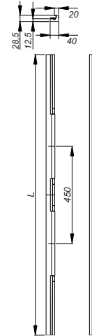
Duschrinne CeraWall Individual N Duo
