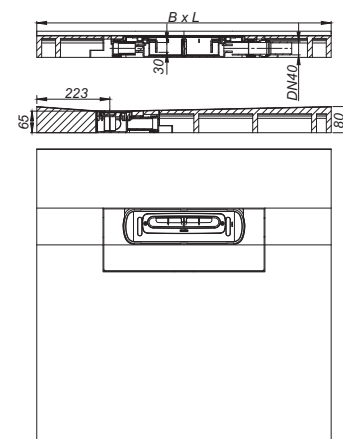
Duschelement DallFlex Floor Plan
